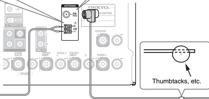
Indoor FM antenna (supplied)
